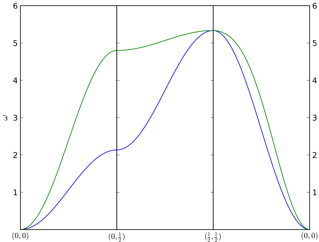
Vibrational frequencies for the k-space path
